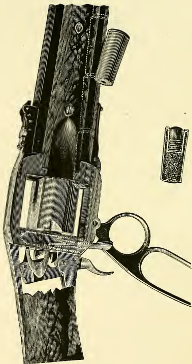
The Needham Magazine Gun and Cartridge.
